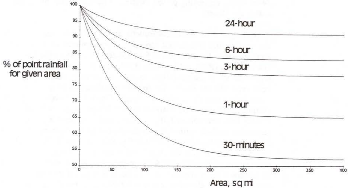
FIG. 2.3.1 Depth-area Adjustment (Source: U.S. Weather Bureau, 1958)
