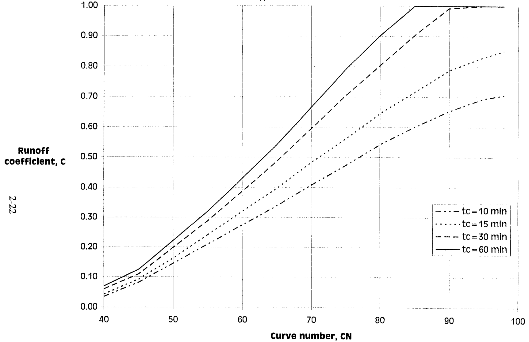
Fig. 2.5.2 Runoff Coefficients for 100-yr Event above 1,640' (SCS type IA storm)
