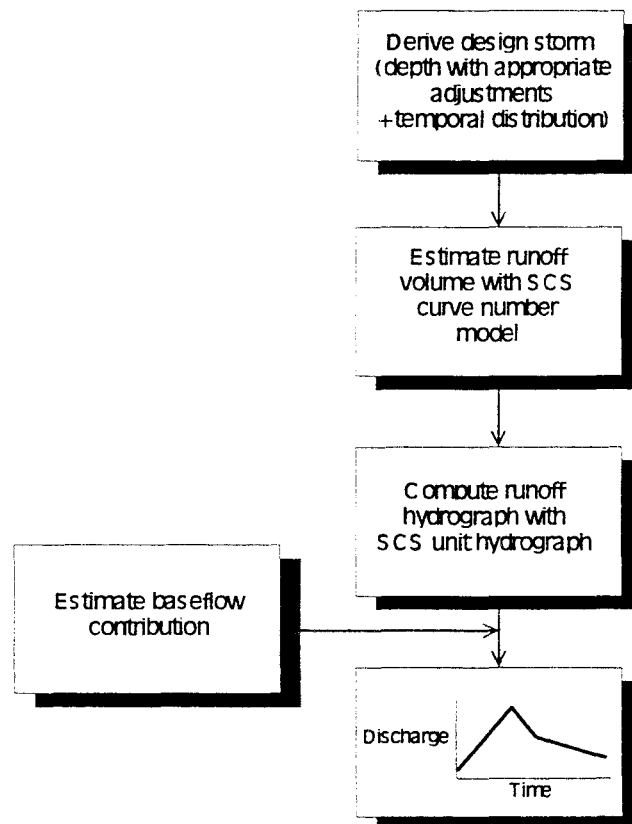
FIG. 2.4.1 Runoff Computation Procedure
