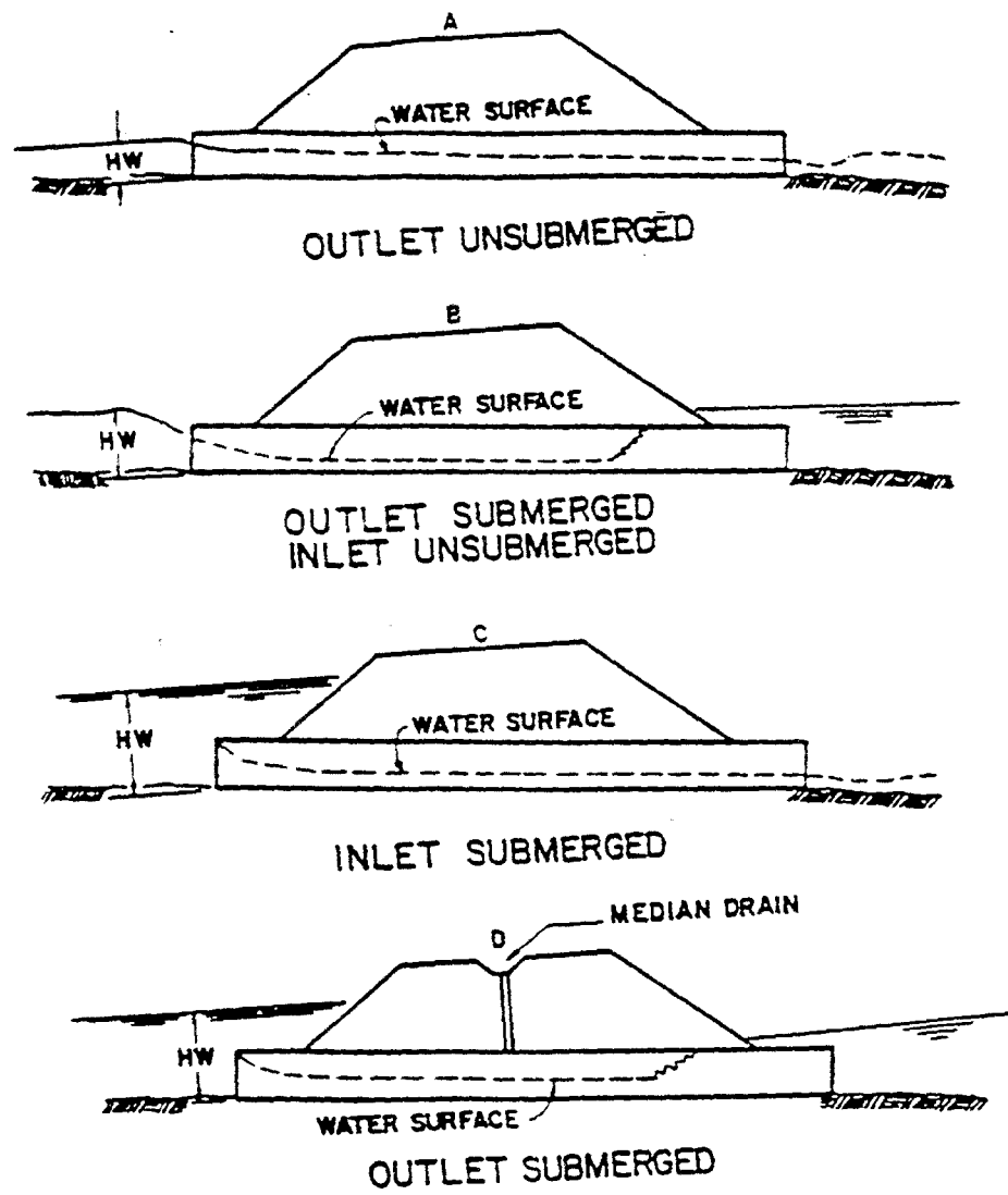
Figure 7.2.1 Schematic Diagram of Types of Inlet Control for Culvert Flow.
