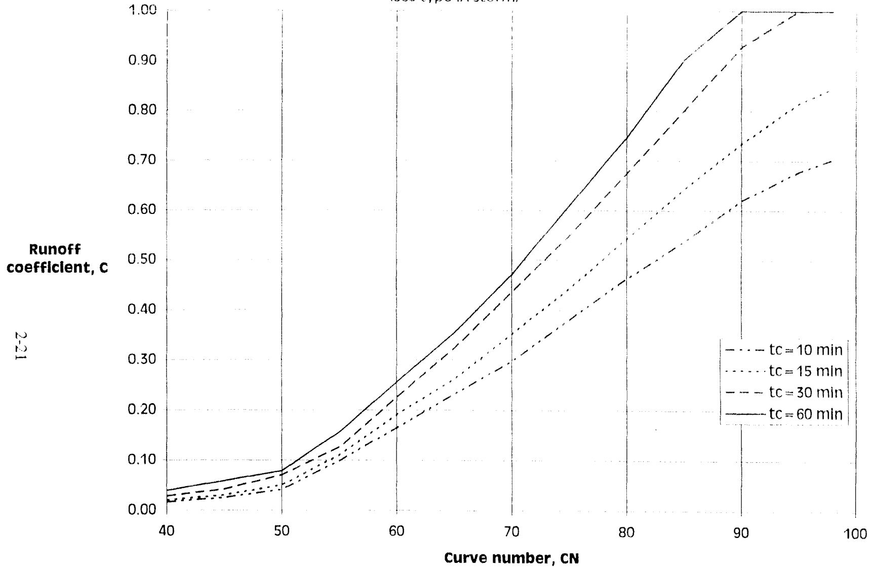
FIG. 2.5.1 Runoff Coefficients for 10-yr Event above 1,640' (SCS type IA storm)
