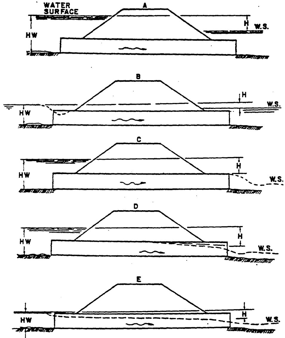
Figure 7.2.2 Schematic Diagram Showing Types of Outlet Control for Culvert Flow.
