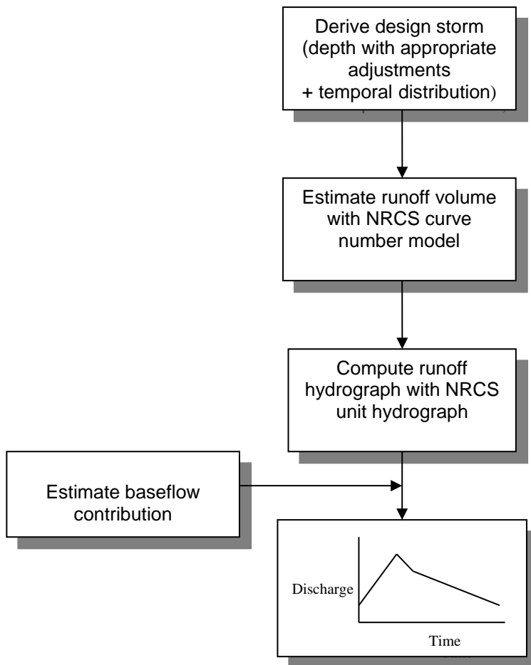
FIG. 2.4.1 Runoff Computation Procedure
