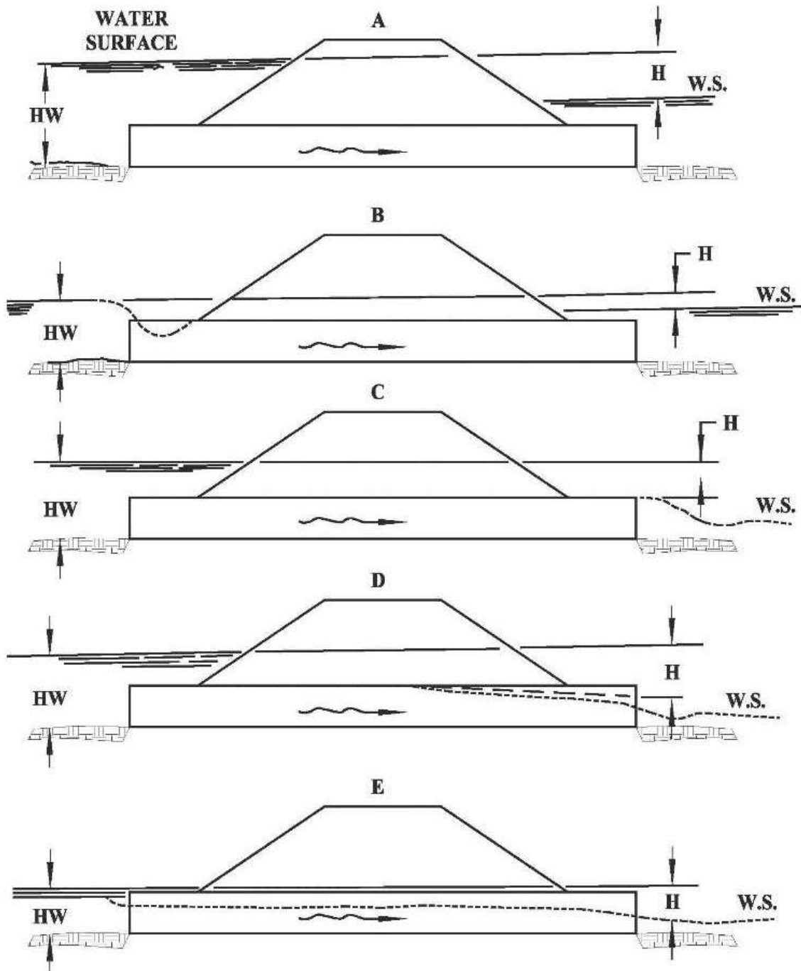
Figure 7.2.2 Schematic Diagram Showing Types of Outlet Control for Culvert Flow. (Source: FHWA, 2005)
