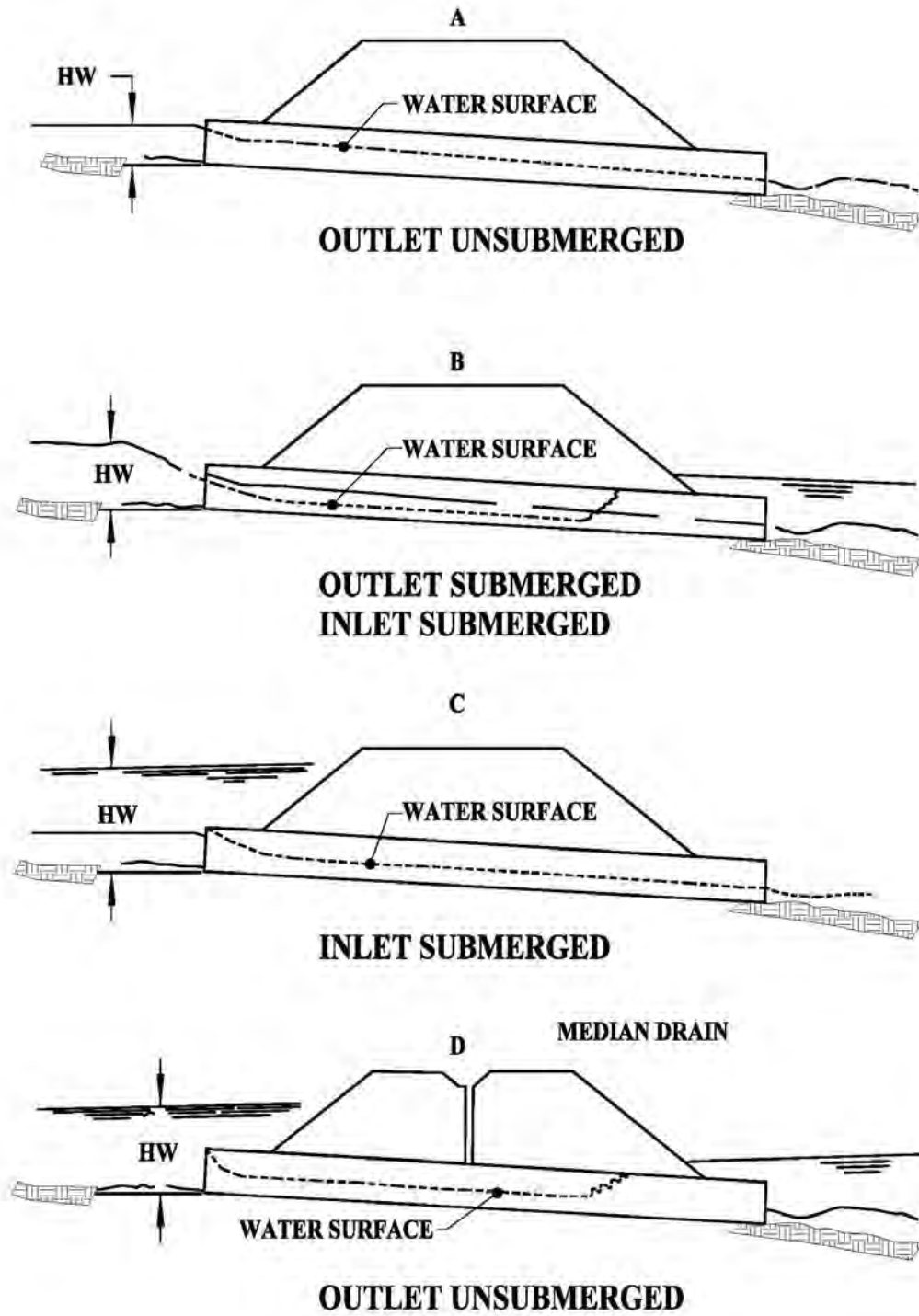
Figure 7.2.1 Schematic Diagram of Types of Inlet Control for Culvert Flow. (Source: FHWA, 2005)
