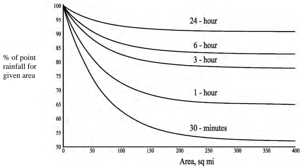
FIG. 2.3.1 Depth-area Adjustment (Source: U.S. Weather Bureau, 1958)
