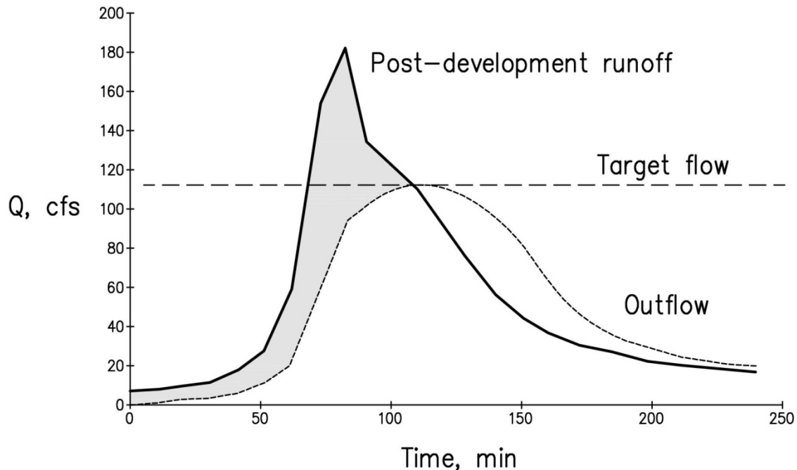
Fig. 5.2.1 Impact of Storage
