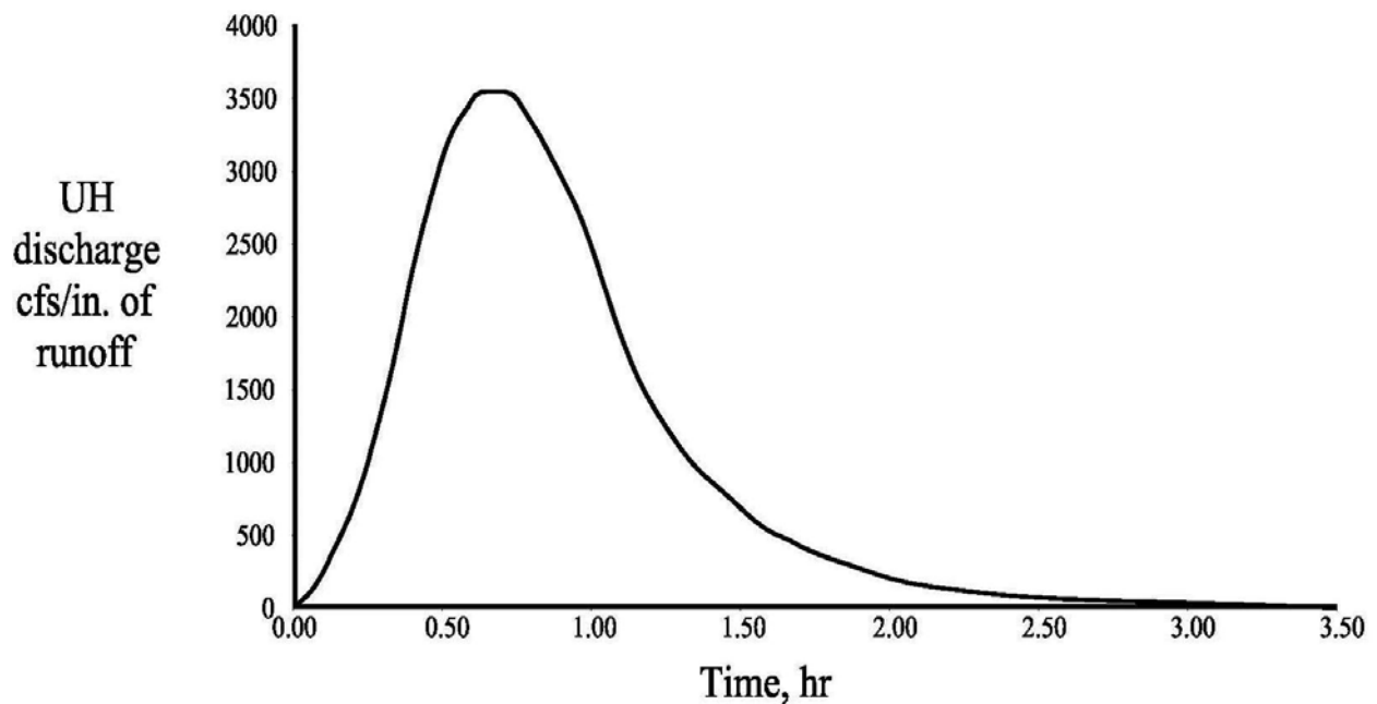
FIG. 2.4.2 Example of 10-min UH for 5 sq mi Catchment
