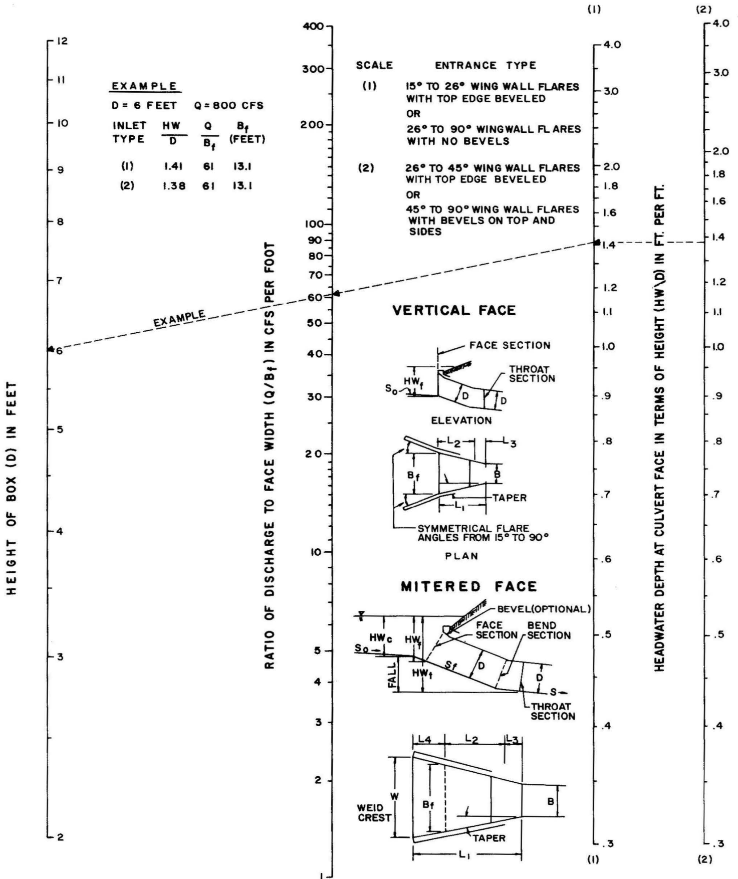
FACE CONTROL FOR BOX CULVERTS WITH SLOPE TAPERED INLETS
