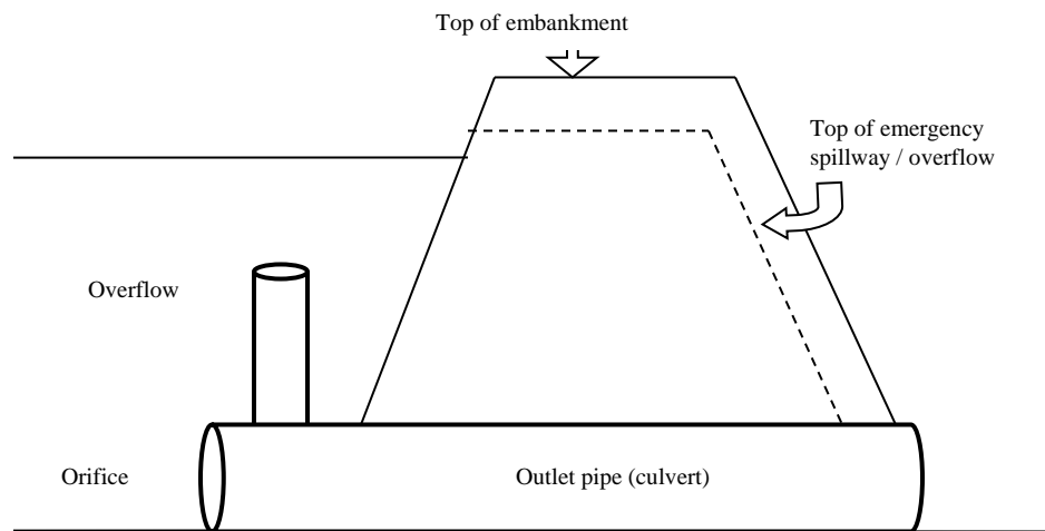
Fig. 5.2.2 Typical Detention Structure
