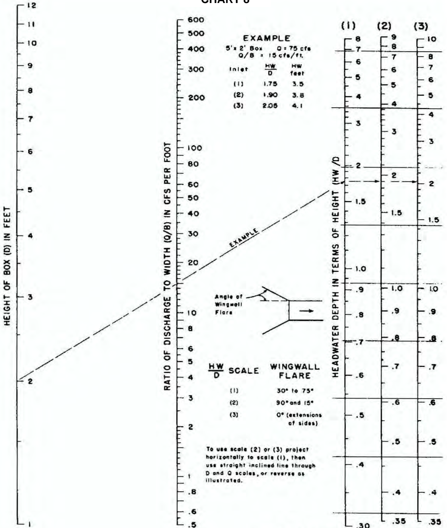
HEADWATER DEPTH FOR BOX CULVERTS WITH INLET CONTROL
