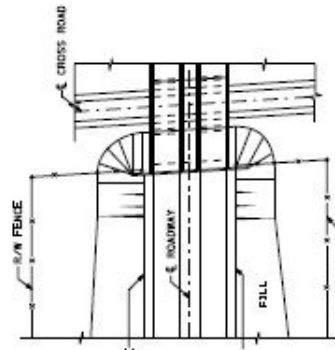
PLAN OF ROADWAY - UNDERCROSSING
