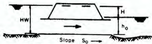
SUBMERGED OUTLET CULVERT FLOWING FULL
