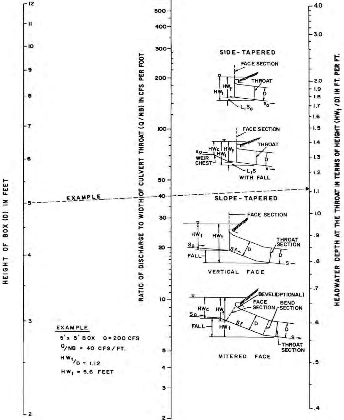
THROAT CONTROL FOR BOX CULVERTS WITH TAPERED INLETS
