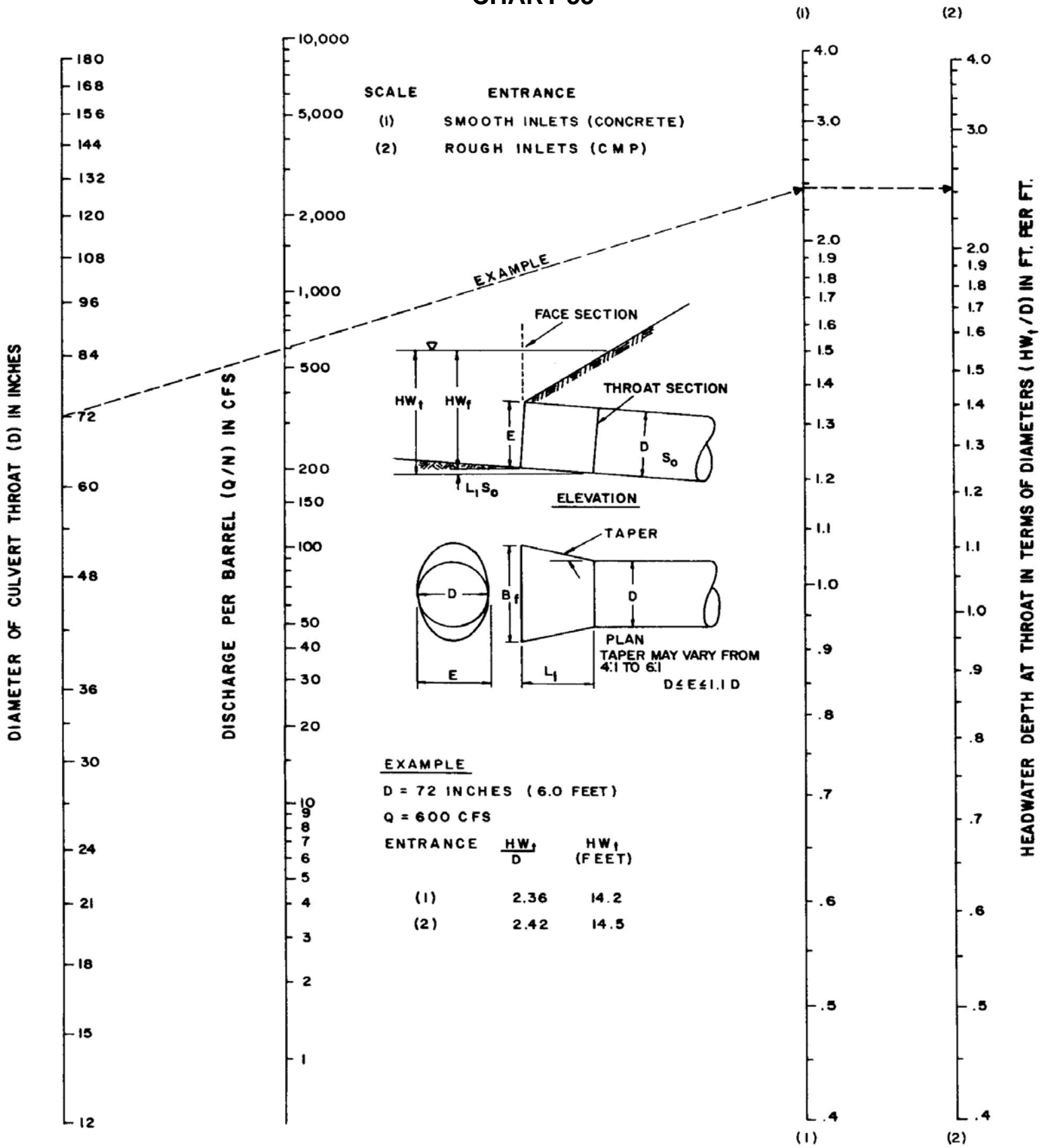
THROAT CONTROL FOR SIDE-TAPERED INLETS TO PIPE CULVERT (CIRCULAR SECTION ONLY)
