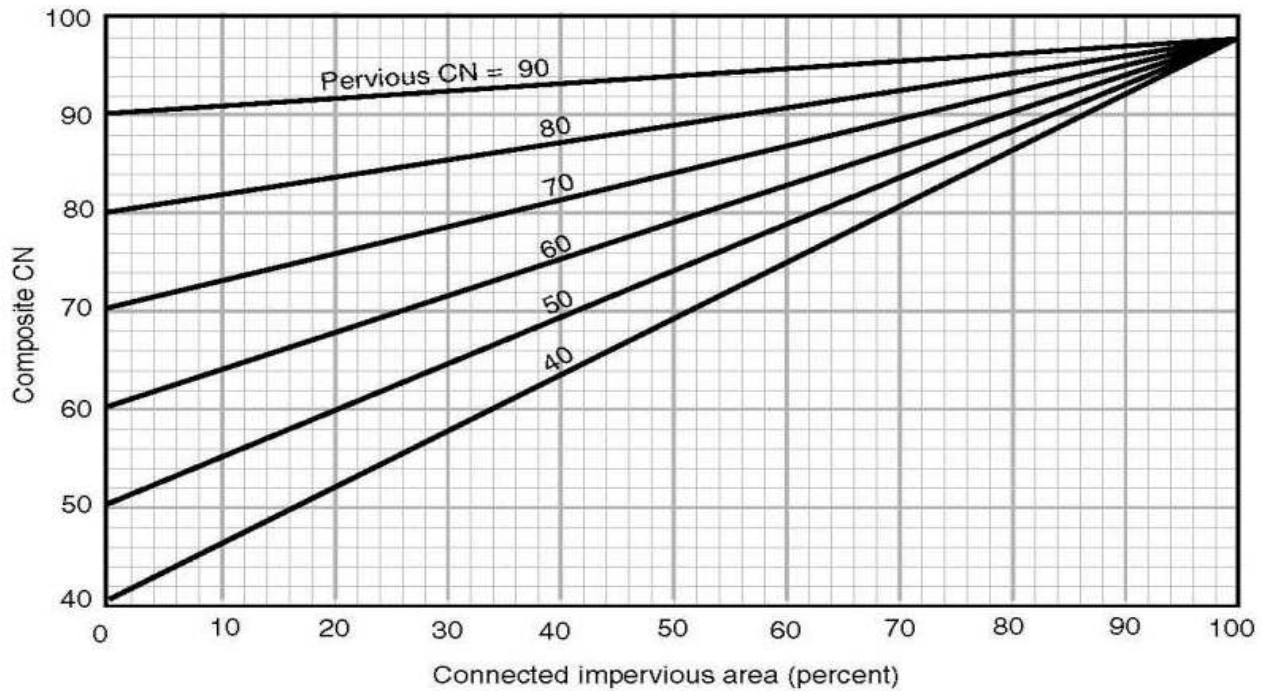
Figure 2-3. – Composite CN with connected impervious area.
