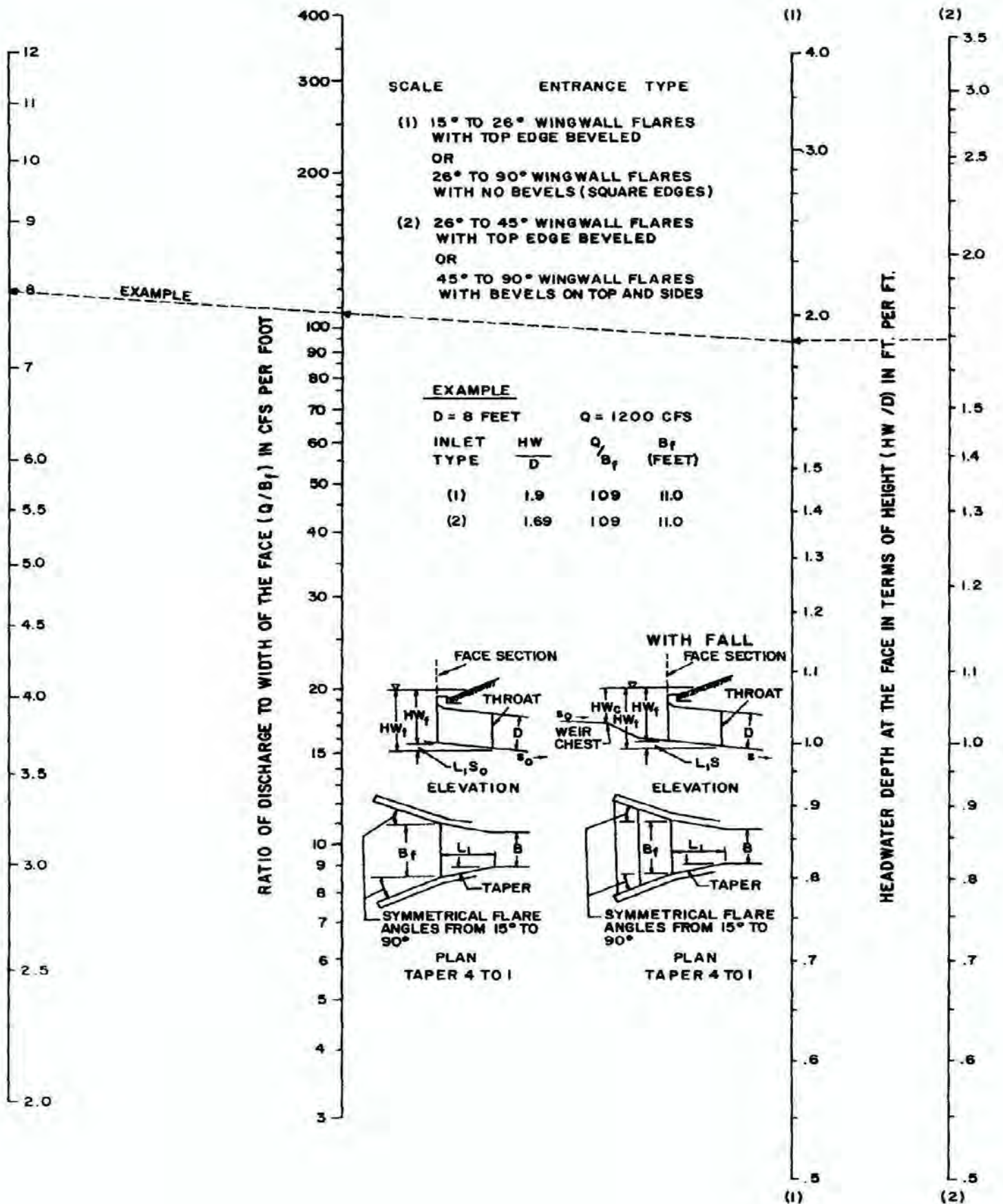
FACE CONTROL FOR BOX CULVERTS WITH SIDE TAPERED INLETS
