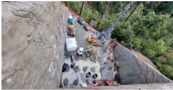
12/20/23 – Pier 3 CIDH Piles 25 of 35 Piles Completed
