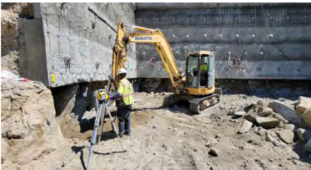
8/17/23 – Pier 2 Structure Excavation – Last Lift
