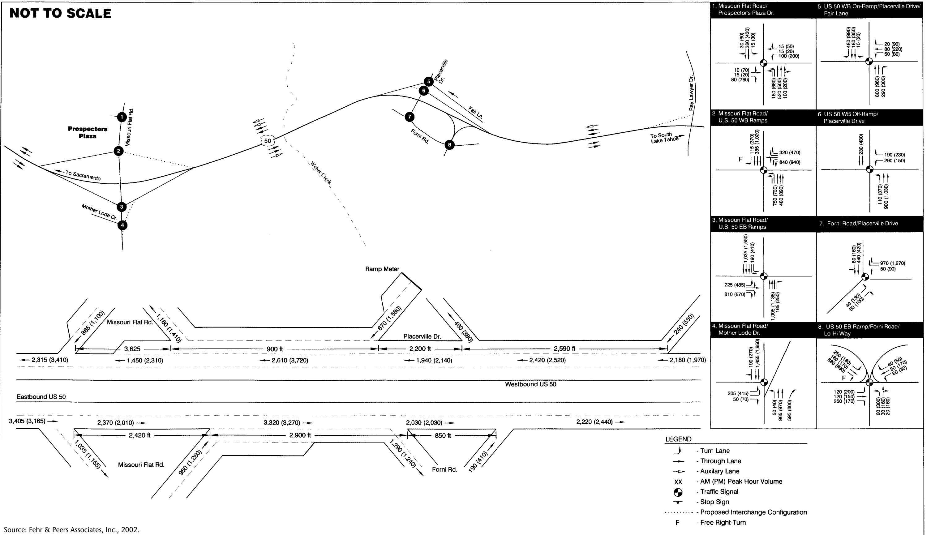
Figure 3.4-4 Six-Lane Diamond Interchange Geometrics, Traffic Control, and Peak Hour Volumes - 2025 Conditions
