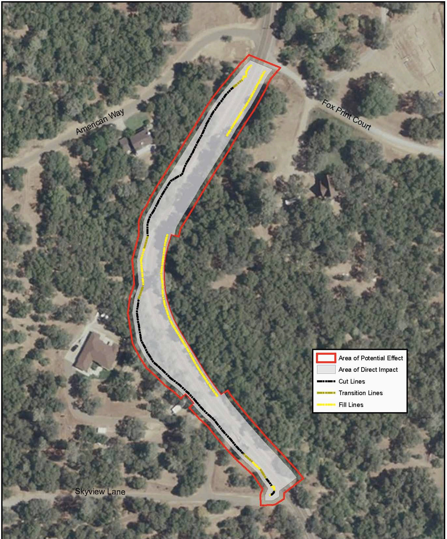
Figure 2: Proposed Project (Segment 1) Cold Springs Road Realignment Project
